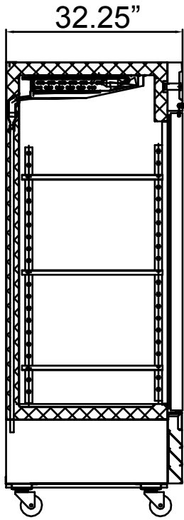
SECTION VIEW
